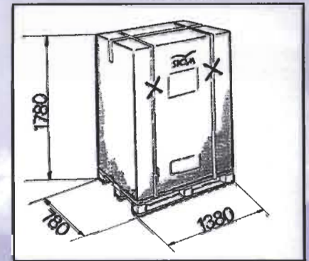
MACHINE PACKED IN STANDING POSITION
